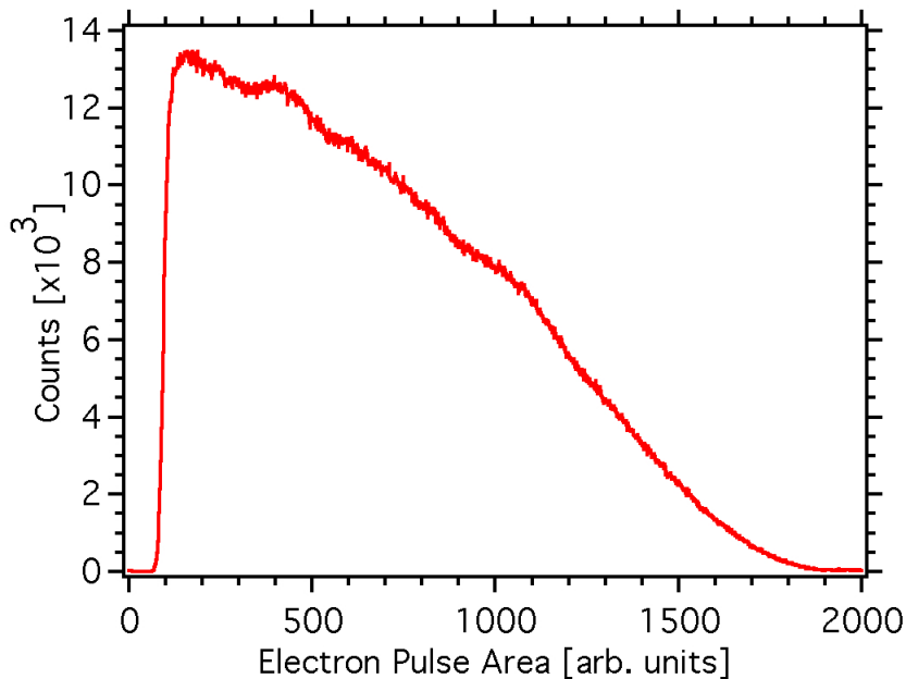
Figure 4.5: Histogram of the electron area from valid electron-delayed proton trigger events. This area is relatable to the electron energy deposited in the SBD. The skew shaped is due to electron backscatter. The features at channels 400 and 1100 are believed to be photon backgrounds.
