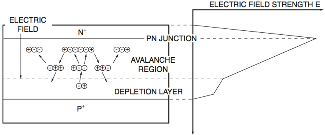
Figure 3.5: Semiconductor layout for a typical APD with the internal electric field felt by the resulting carriers [3].
