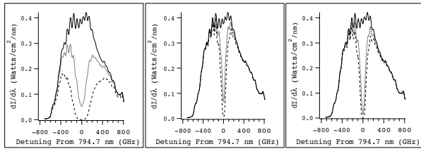
Figure 3: Profile of intensity vs. wavelength for a typical \text{GaAl}^x\text{As}^{1-x} LDA (from Optopower Corp.), indicated by a solid line. The total power output per laser is about 15 watts. The dotted and dashed lines show the laser profile 5 cm and 10 cm into the cell, respectively, for cell parameters of: 10 amagat of ^3\text{He} and 0.1 amagat \text{N}_2 at 180°C (left); 0.1 amagat of ^{129}\text{Xe} , 0.2 amagat \text{N}_2 , and 2.7 amagat He at 110°C (center); and 2.2 amagat of ^{129}\text{Xe} , 0.2 amagat \text{N}_2 , and 0.5 amagat He at 110°C (right).
