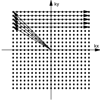
Figure 8: Sampling of k -space by the gradient echo pulse sequence. The phase-encode gradient varies from scan to scan and allows complete sampling of k_y . The readout gradient is prephased to -k_x^{max} and runs to +k_x^{max} . The resolution of the image is determined by the value of k_x^{max} and the field-of-view of the image is determined by the step size in k -space.
