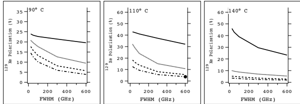
Figure 4: Calculated ^{129}\text{Xe} polarization as a function of the LDA line width (FWHM). For each temperature, curves for 0.13 amagat, 0.65 amagat, 1.3 amagat, and 2 amagat of ^{129}\text{Xe} are shown from top to bottom, respectively. A constant total density of 2.8 amagat is maintained by loading with helium buffer gas. The solid dot on the 110° shows the measured ^{129}\text{Xe} polarization reported by [Rosen et al., 1999].
