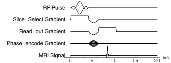
Figure 7: Gradient echo imaging (GRAS or FLASH). Magnetization is sampled in k_x and k_y as shown in figure 8. A two-dimensional Fourier transform of uniformly sampled k-space creates the image.
