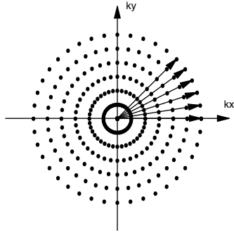
Figure 6: Sampling of k-space by back-projection imaging. In this example, we illustrate just the first few sampled rays obtained by adjusting the gradients according to equation 36
