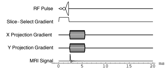
Figure 5: Pulse sequence for Back Projection imaging in two-dimensions. The slice-selective gradient and the frequency-selective RF pulse only excite spins in a slice or slab along the z-axis. The half sinc slice-selective pulse does not require that the transverse magnetization be refocused. The two projection gradients are varied in a sinusoidal pattern.
